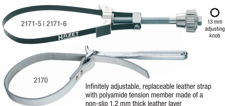
2171-5 | 2171-6 Infinitely adjustable, replaceable steel strap
